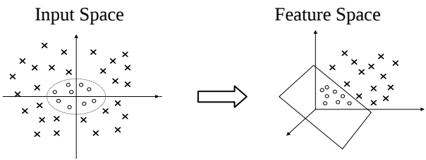
FIGURE 1: Mapping nonlinear data to a higher dimensional feature space where a linear separating hyperplane can be found. When mapped into a feature space via the non-linear map \Phi(x) = (z_1, z_2, z_3) = ([x]_1^2, [x]_2^2, \sqrt{2}[x]_1[x]_2)
